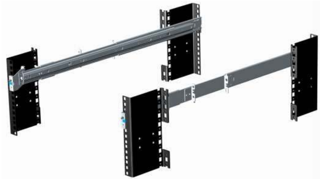
Figure 10. Static rails
